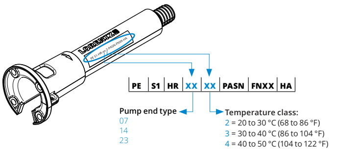
Figure 1: Pump end naming
